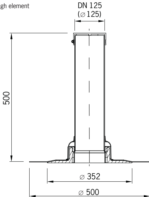
Reach-through element \varnothing DN 125
