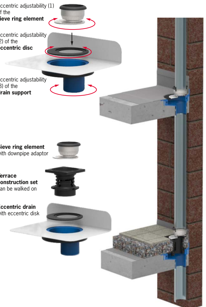
Eccentric drain with sieve ring attachment DN 70
