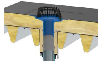
Compact fire protection drain DN 100 with inserted Eco drain top part in the trapezoid sheet roof with insulated roof construction.
