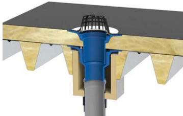
Fire protection cladding with universal drain and extension element in trapezoidal sheet roofs with insulated roof construction.
